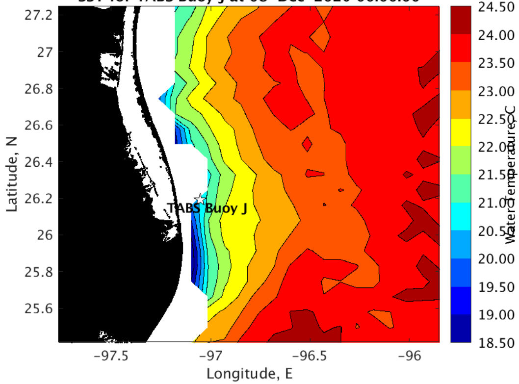
SST for TABS Buoy J at 08-Dec-2020 00:00:00
